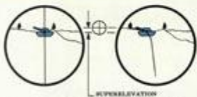
A new stereoscopic fire control development by Cadillac Gage aims gun with proper super-elevation for a hit when sights are laid on target. There are no moving parts in this system.
